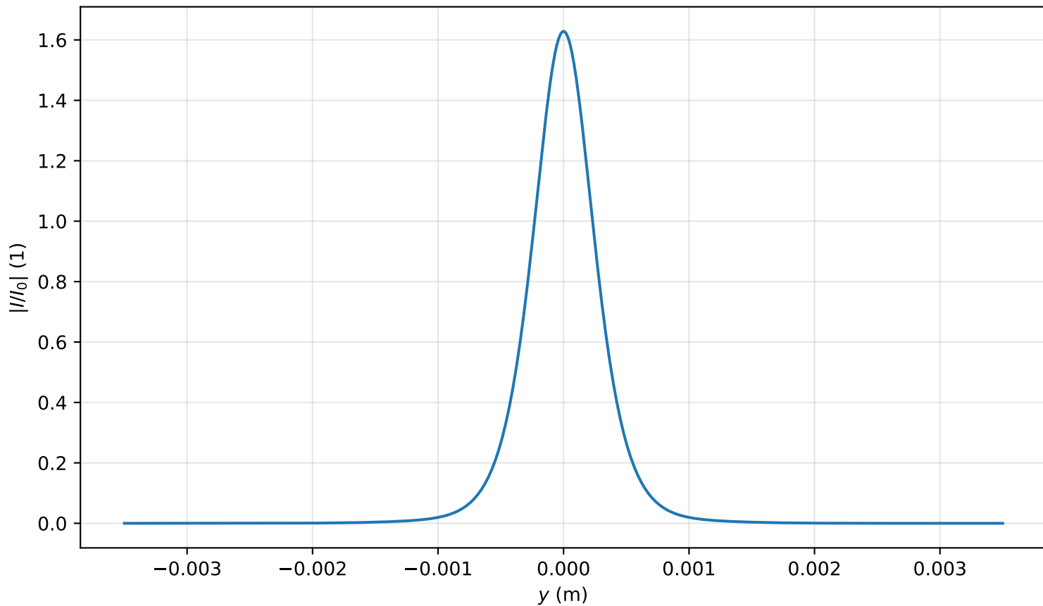
Intensity profile I(x = 0, y, z = 2.388)/I_0 , P_{in}=0.9P_{cr} , artificial time
